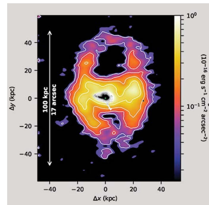
David Rupke's diagram of outflow from Makani
