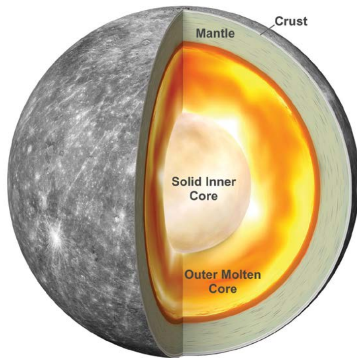
A cutaway view of the planet Mercury's interior. The inner core is solid; the outer core is liquid. They both have an unusually large concentration of iron compared to the cores of the other terrestrial planets. Above that is a solid anticrost (orange-tan layer in this graphic). A silicate-rich mantle supports a thin crust on the top of the planet. Convection in the outer mantle acts a dynamo to generate Mercury's magnetic field. Credit: NASA's Goddard Space Flight Center.
