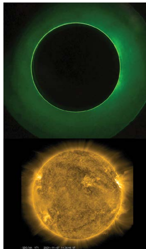
Figure 1: Hripcsak's image at top, compared to a Solar Dynamics Observatory image from about the same time.
