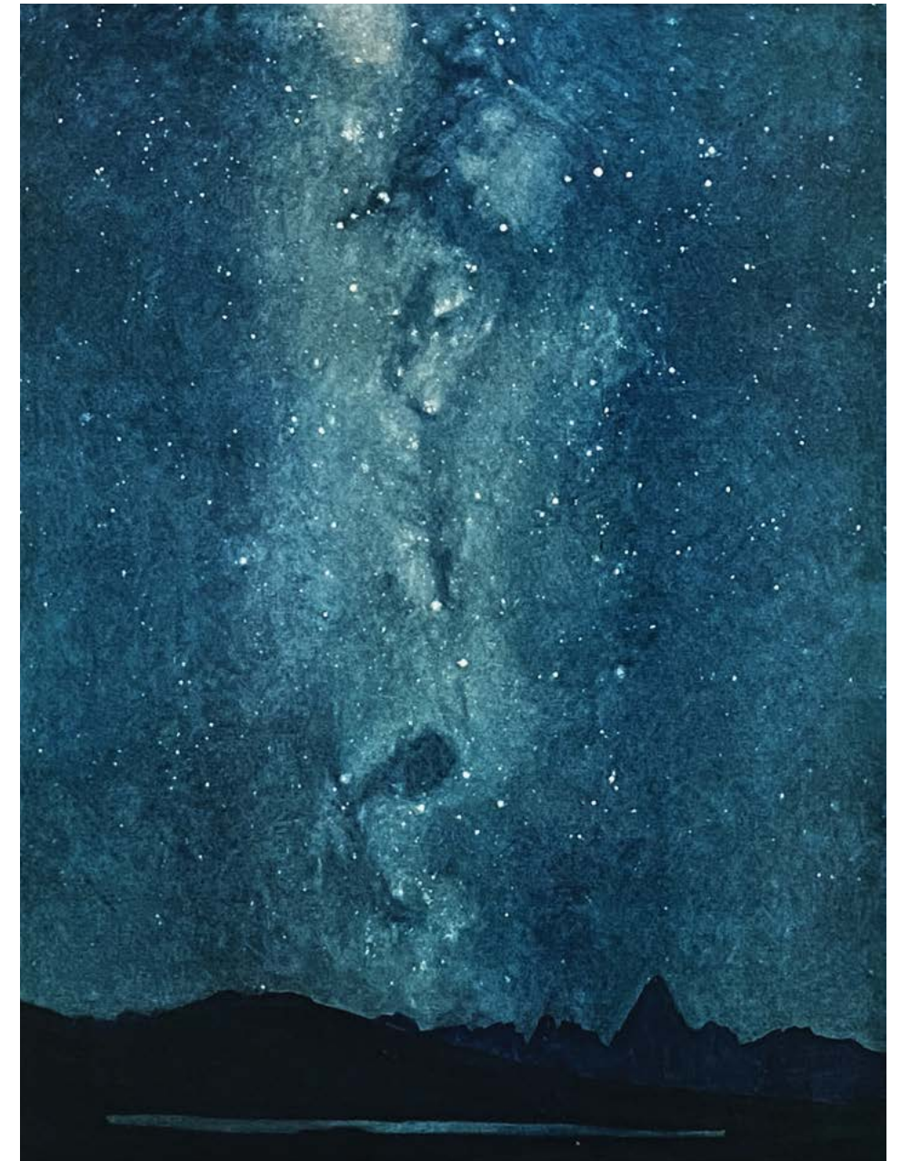
"The Milky Way from Sagittarius to Crux," The Sky Magazine, Amateur Astronomers Association of New York.
