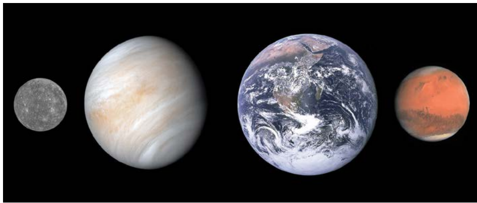
The four terrestrial planets, Mercury, Venus, Earth, and Mars, are shown here at their relative sizes. These rocky planets are vastly different from the gas giants further out in the Solar System. Mercury has the largest core, occupying 55 percent of the planet by volume, and it is a liquid outer core surrounding a solid inner core. Venus has a core that occupies 14 percent and it is probably solid. Earth's core occupies 17 percent of the planet's volume and is a liquid outer core over a solid inner core. Mars has a core that is 16 percent of the volume of the planet and is liquid. Credits: Mercury, Venus, and Earth images from NASA; Mars image ESA/MPS/UPD/LAM/IAA/RSSD/INTA/UPM/DASP/IDA
