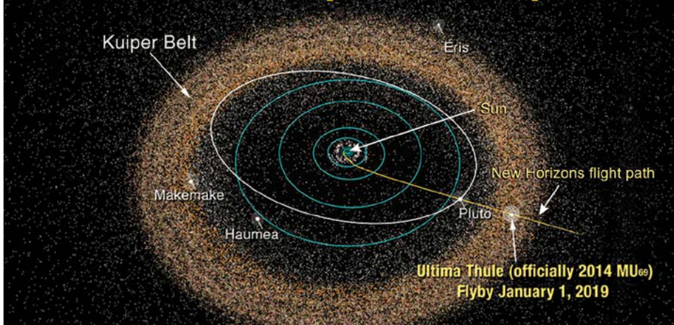
The Kuiper Belt is much larger than the main asteroid belt (represented by the white spots inside the orbit of Jupiter). Its members are also icy and not rocky, so if they get near the Sun, they release dust and gas to become comets. This belt extends outward from Neptune. Pluto and Arrokoth (2014 MU69 or, informally, Ultima Thule) are in the Kuiper Belt, but it extends far beyond both. Image credit: NASA/Johns Hopkins University Applied Physics Laboratory/Southwest Research Institute
