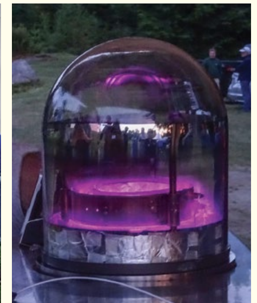
Alan Ward drew a crowd with his portable coating machine; he aluminized several conventioners' mirrors on site. Right: The glow of pumpdown at twilight. Photos by Patrick Dodson.
