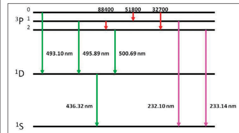
Forbidden and permitted electron transitions in the oxygen atom (Wikipedia user Cepheiden, en.wikipedia.org/wiki/Doubly_ionized_oxygen#/media/File:Oiii-linesp.svg)
