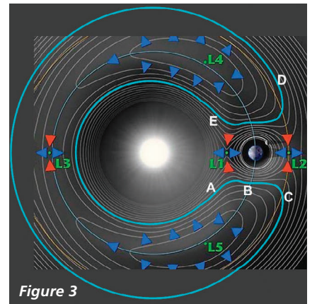
Figure 3 A minor planet in a horseshoe orbit is trapped by Earth's gravity. This view shows the object's motion relative to the Earth over an extended period (for 2002 AA 29 over two centuries). At point A, the object is in an orbit closer to the Sun than the Earth's orbit, so it is moving faster than the Earth. Between L5 (Lagrange 5) and the Earth, the object is pulled by the Earth's gravity, speeding it up. This moves it toward a higher orbit through point B to point C. The object is now in a more distant, slower orbit, so it starts to fall behind the Earth. It moves all the way around the Sun to the leading side of the Earth (point D) where the process reverses. Earth's gravity slows the object and it drops into a closer, faster orbit (point E) and starts to outrun the Earth again. (NASA/Jet Propulsion Laboratory/California Institute of Technology)
